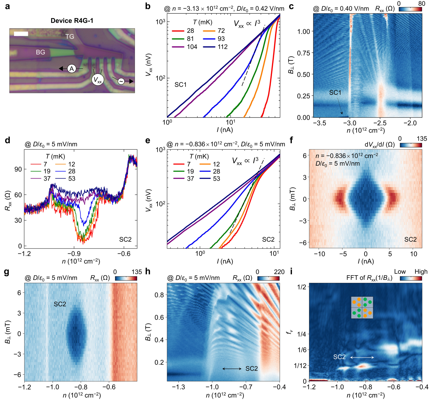
Extended Data Fig. 2 | Additional data for SC1 and SC2 in R4G. a , Optical image of Device R4G-1 with a representative measurement configuration. Scale bar: 3 \mu\text{m} . b , Voltage V_{xx} versus current I at varied temperatures for the SC1 of R4G. c , R_{xx} as a function of n and B_{\perp} , covering the density range of the SC1. The data in c was used for the Fourier transform in Fig. 1f. d , R_{xx} as a function of n at varied temperatures for the SC2 of R4G. e , Voltage V_{xx} versus current I at varied temperatures for the SC2. The dashed line denotes when V_{xx} is proportional to I^3 , corresponding to the BKT transition temperature T_{\text{BKT}} \approx 19 \text{ mK} . f , Differential
