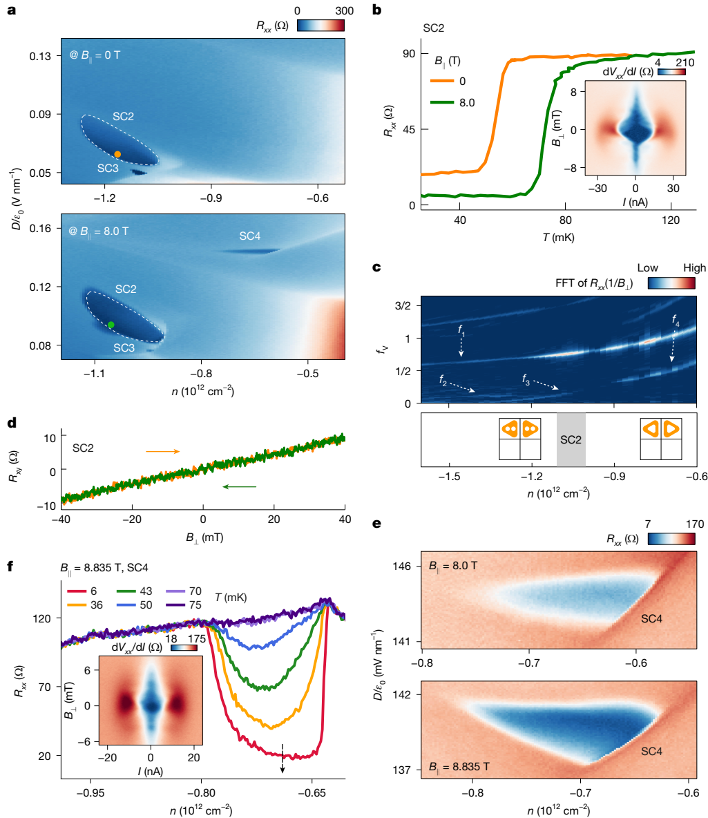
Fig. 2 | SC2 and SC4 in R5G, respectively, enhanced and induced by B_{\parallel} . a , R_{xx} maps at B_{\parallel} = 0 T (top) and 8 T (bottom). Whereas SC3 survives, SC2 is enlarged, and SC4 is induced by B_{\parallel} . For comparison, the boundary of SC2 at B_{\parallel} = 0 T is drawn as white dashed curves. b , R_{xx} as functions of T at the (n, D) point (indicated as circles in a ) with the minimal resistance at each field. The transition temperature is increased by applying B_{\parallel} . The inset shows differential resistance as a function of I and B_{\perp} for SC2 at B_{\parallel} = 6.5 T. Fraunhofer-like modulations are observed. c , Fast Fourier transform of R_{xx}(1/B_{\perp}) as a function of n and f_v . Around SC2, f_2 and f_3 have merged and the relation f_1 - 2f_3 \approx 1/2 holds, suggesting its normal state is a half-metal with an annular-shaped Fermi surface. d , R_{xy} as a
