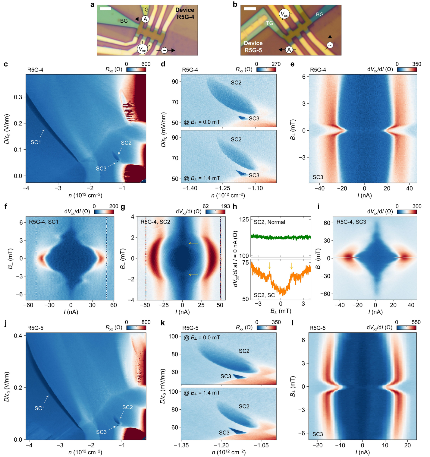
Extended Data Fig. 5 | Reproducibility of SC in R5G from Device R5G-4 and R5G-5. a, b , Optical image of Device R5G-4 (a) and R5G-5 (b) with representative measurement configurations. Scale bar: 3 \mu\text{m} . c , R_{xx} as a function of n and D/\epsilon_0 for Device R5G-4. All three SCs in Fig. 1a are reproduced. d , R_{xx} as a function of n and D/\epsilon_0 focusing on SC2 and SC3 at B_{\perp} = 0.0 (top) and 1.4 mT (bottom). Area in the n - D space occupied by SC3 increased by a nonzero B_{\perp} . e , Differential resistance as a function of I and B_{\perp} for SC3 ( n = -1.16 \times 10^{12} \text{ cm}^{-2} , D/\epsilon_0 = 55 \text{ mV/nm} ), showing the increase of critical current by small B_{\perp} . f-i , Differential resistance as a function of I and B_{\perp} for SC1 ( n = -3.57 \times 10^{12} \text{ cm}^{-2} , D/\epsilon_0 = 0.225 \text{ V/nm} ) (f), SC2 ( n = -1.17 \times 10^{12} \text{ cm}^{-2} , D/\epsilon_0 = 67 \text{ mV/nm} ) (g) and SC3 ( n = -1.16 \times 10^{12} \text{ cm}^{-2} , D/\epsilon_0 = 55 \text{ mV/nm} ) (i)
