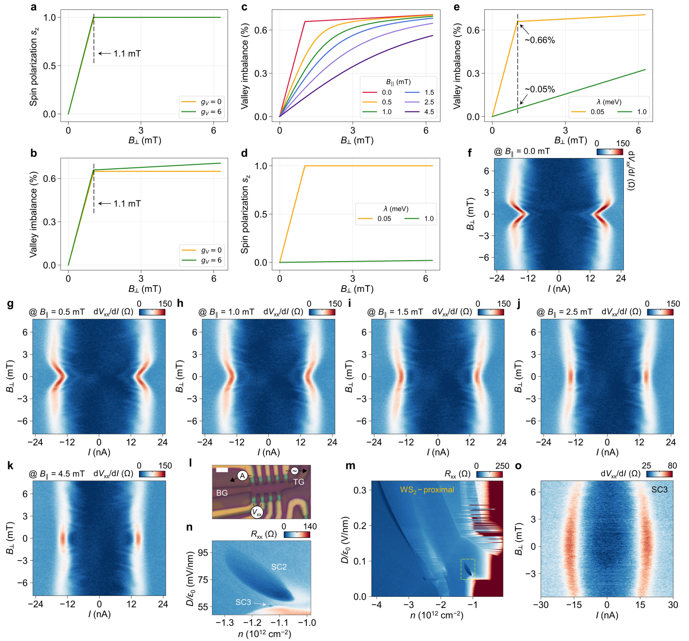
Extended Data Fig. 9 | Calculations for the enhancement of SC3 and supporting experimental results. a,b , Spin polarization s_z ( a ) and valley imbalance normalized by n_0 ( b ) as functions of a perpendicular magnetic field for bare RSG with g_V = 0 and 6. The optimal value of B_\perp , calculated to be 1.1 mT, is mostly independent of g_V . c , Valley imbalance normalized by n_0 under varied B_\parallel as functions of B_\perp . The increase in the valley imbalance by B_\perp gets slower by applying B_\parallel , which is consistent with the experimental observations. d,e , Effect of the proximitized SOC on the spin polarization ( d ) and valley imbalance ( e ). When
