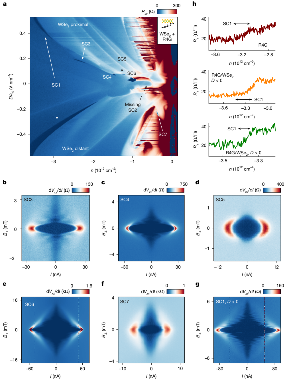
Fig. 4 | Proliferation of SC in R4G by proximitized SOC effects. a , R_{xx} map of a R4G/WSe 2 device. Five new states (SC3–7) emerge while SC2 is suppressed. The names of SCs follow the convention of Fig. 1b. b–g , Differential resistance as a function of I and B_{\perp} for SC3 ( n = -2.356 \times 10^{12} \text{ cm}^{-2} , D/\epsilon_0 = 0.18 \text{ V nm}^{-1} ), SC4 ( n = -1.482 \times 10^{12} \text{ cm}^{-2} , D/\epsilon_0 = 0.072 \text{ V nm}^{-1} ), SC5 ( n = -1.242 \times 10^{12} \text{ cm}^{-2} , D/\epsilon_0 = 0.072 \text{ V nm}^{-1} ), SC6 ( n = -1.00 \times 10^{12} \text{ cm}^{-2} , D/\epsilon_0 = 0.026 \text{ V nm}^{-1} ), SC7 ( n = -0.38 \times 10^{12} \text{ cm}^{-2} , D/\epsilon_0 = -0.24 \text{ V nm}^{-1} ) and SC1 ( n = -3.25 \times 10^{12} \text{ cm}^{-2} ,
