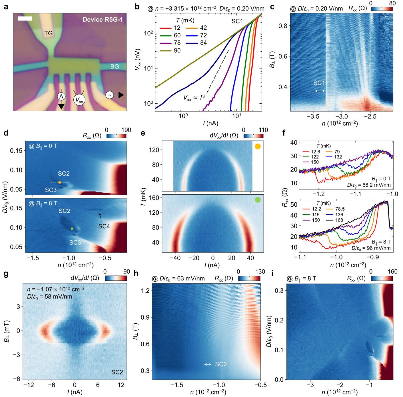
Extended Data Fig. 1 | Additional data for SC1 and SC2 in R5G. a , Optical image of Device R5G-1 with a representative measurement configuration. Scale bar: 3 \mu\text{m} . b , Voltage V_{xx} versus current I at varied temperatures for the SC1 of R5G. c , R_{xx} as a function of n and B_{\perp} , covering the density range of the SC1. The data in c was used for the Fourier transform in Fig. 1e. d , R_{xx} maps at B_{||} = 0.0 (top) and 8.0 (bottom) T from Device R5G-1. While SC3 is robust, SC2 is enlarged and SC4 is induced by B_{||} . e , Differential resistance as a function of I and T at the orange and green dot positions in d . Both I_c and T_{BK\Gamma} are enhanced by B_{||} . f , R_{xx} as a function of n at varied temperatures along the dashed lines in d . The R_{xx}
