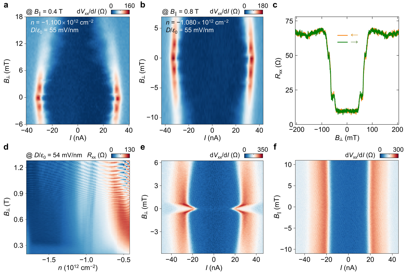
Extended Data Fig. 8 | Additional data for SC3 in RSG. a,b , Differential resistance as a function of I and B_{\perp} for B_{\parallel} = 0.4 T ( a ) and B_{\parallel} = 0.8 T ( b ). B_{\perp} -induced enhancement for SC3 disappeared under a high enough in-plane field. c , R_{xx} as a function of B_{\perp} in the forward and backward scanning directions for SC3 ( n = -1.132 \times 10^{12} \text{ cm}^{-2} , D/\epsilon_0 = 54 \text{ mV/nm} ) at the base temperature. There is no hysteretic behavior observed, implying the absence of orbital magnetism in
