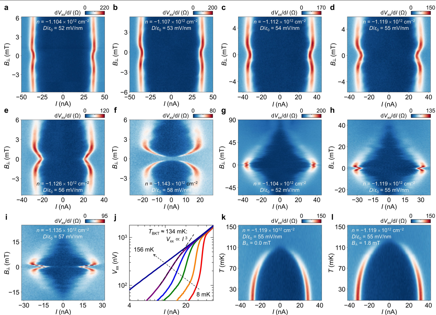
Extended Data Fig. 7 | T - and B_{\perp} -dependent measurements on SC3 in Device R5G-1. a-f , Differential resistance as a function of I and B_{\perp} at different (n, D) points. The enhancement of SC3 by B_{\perp} is observed globally across its phase space. g-i , Differential resistance as a function of I and B_{\perp} at different (n, D) points for a wider range of the magnetic field. Fraunhofer-like patterns arising from quantum interference are observed in i which is adjacent to the phase boundary of SC3, and they become fainter as D/\epsilon_0 decreases. j , V_{xx} versus current I at T = 8 ,
