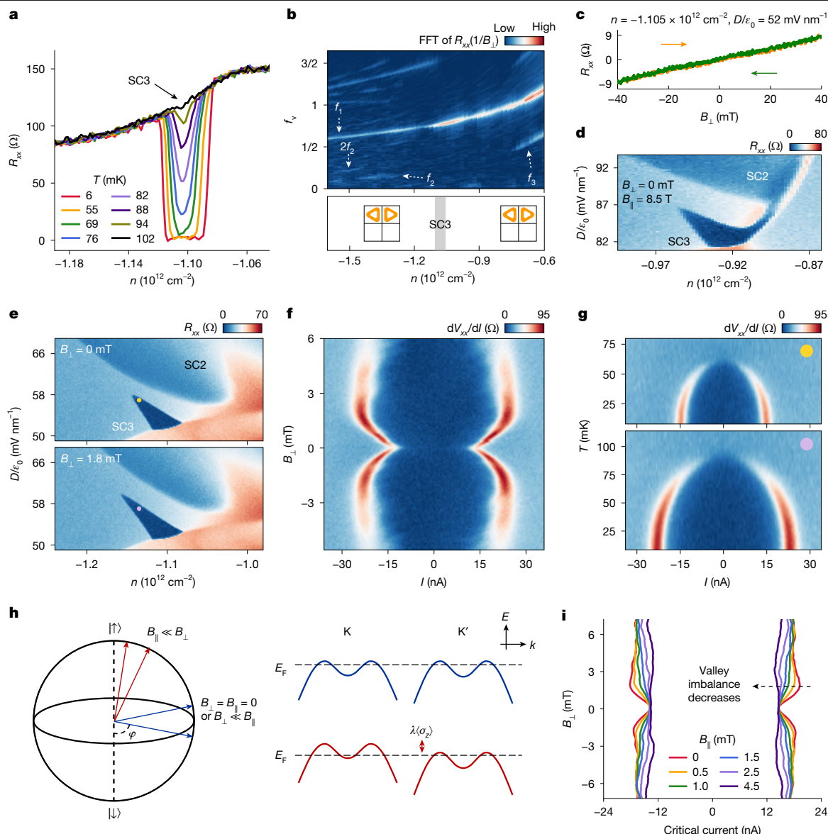
Fig. 3 | SC3 in RSG enhanced by B_{\perp} . a , R_{xx} as a function of n at D/\epsilon_0 = 49.61 \text{ mV nm}^{-1} and varied temperatures. The resistance vanishes as T decreases. b , Fast Fourier transform of R_{xx}(1/B_{\perp}) as a function of n and f_v , suggesting SC3 is developed from a half-metal with an annular-shaped Fermi surface. c , R_{xx} as a function of B_{\perp} in the forward and backward scanning directions in the normal state of SC3 ( T = 160 \text{ mK} ). The absence of the anomalous Hall effect indicates zero valley polarization. d , R_{xx} map at B_{\perp} = 0 \text{ mT} and B_{\parallel} = 8.5 \text{ mT} . SC3 features ultrahigh PVR of >34 . e , R_{xx} maps at B_{\perp} = 0 \text{ mT} (top) and 1.8 \text{ mT} (bottom). The SC3 region is enlarged by B_{\perp} . f , Differential resistance as a function of I and B_{\perp} for n = -1.135 \times 10^{12} \text{ cm}^{-2} and D/\epsilon_0 = 57 \text{ mV nm}^{-1} . I_c is increased by small B_{\perp} . g , Differential resistance as a function of I and T for n = -1.135 \times 10^{12} \text{ cm}^{-2} and D/\epsilon_0 = 57 \text{ mV nm}^{-1}
