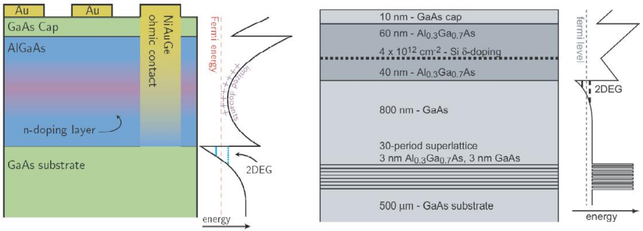
Figure 2.7: Growth profile and bandstructure of typical GaAs heterostructures.
