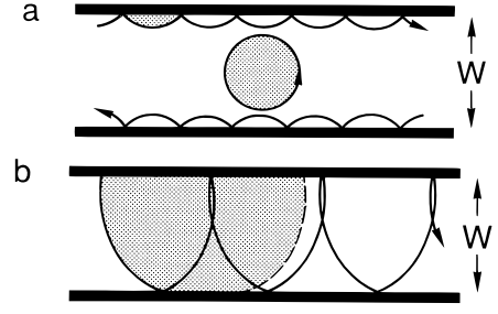
FIG. 41 Classical trajectories in a magnetic field. The flux through the shaded area is quantized according to the Bohr-Sommerfeld rule (3.7). The shaded area in (b) is bounded by the channel walls and the circle formed by the continuation (dashed) of one circular arc of the traversing trajectory.
