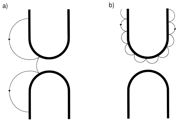
FIG. 51 Illustration of the reduction of backscattering by a magnetic field, which is responsible for the negative magnetoresistance of Fig. 50. Shown are trajectories approaching a constriction without a potential barrier, in a weak (a) and strong (b) magnetic field. Taken from H. van Houten et al., in Ref. 9 .
