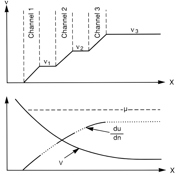
FIG. 94 Schematic drawing of the variation in filling factor \nu , electrostatic potential V , and chemical potential du/dn , at a smooth boundary in a 2DEG. The dashed line in the bottom panel denotes the constant electrochemical potential \mu = V + du/dn . The dotted intervals indicate a discontinuity (energy gap) in du/dn and correspond in the top panel to regions of constant fractional filling factor \nu_p that spatially separate the edge channels. The width of the edge channel regions shrinks to zero in the integer QHE, since the compressibility \chi of these regions is infinitely large in that case. Taken from C. W. J. Beenakker, Phys. Rev. Lett. 64 , 216 (1990).
