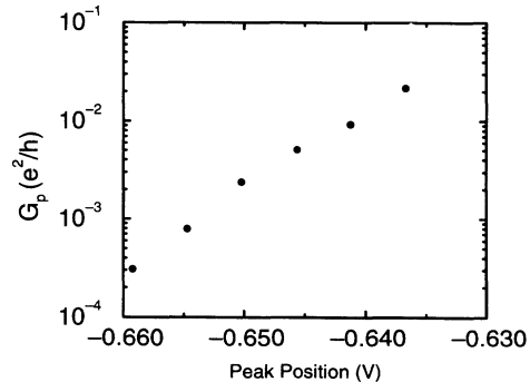
FIG. 3. The peak conductance as a function of peak position at 1 \text{ K} , from the data of Fig. 2, on a logarithmic scale showing the exponential increase of the conductance. This is consistent with the idea that the conductance increases with V_g because the energy difference between the Fermi energy and the barrier decreases.
